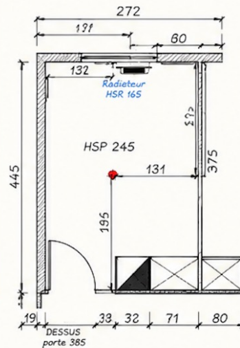
PLAN EXISTANT
